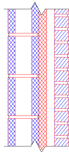
16" Thick Insulated Wall
